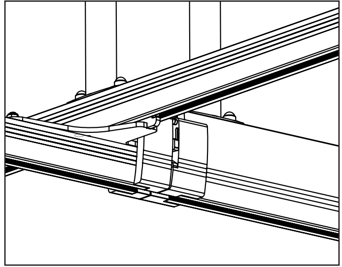
Transfer – gekoppelde traversekoppeling
